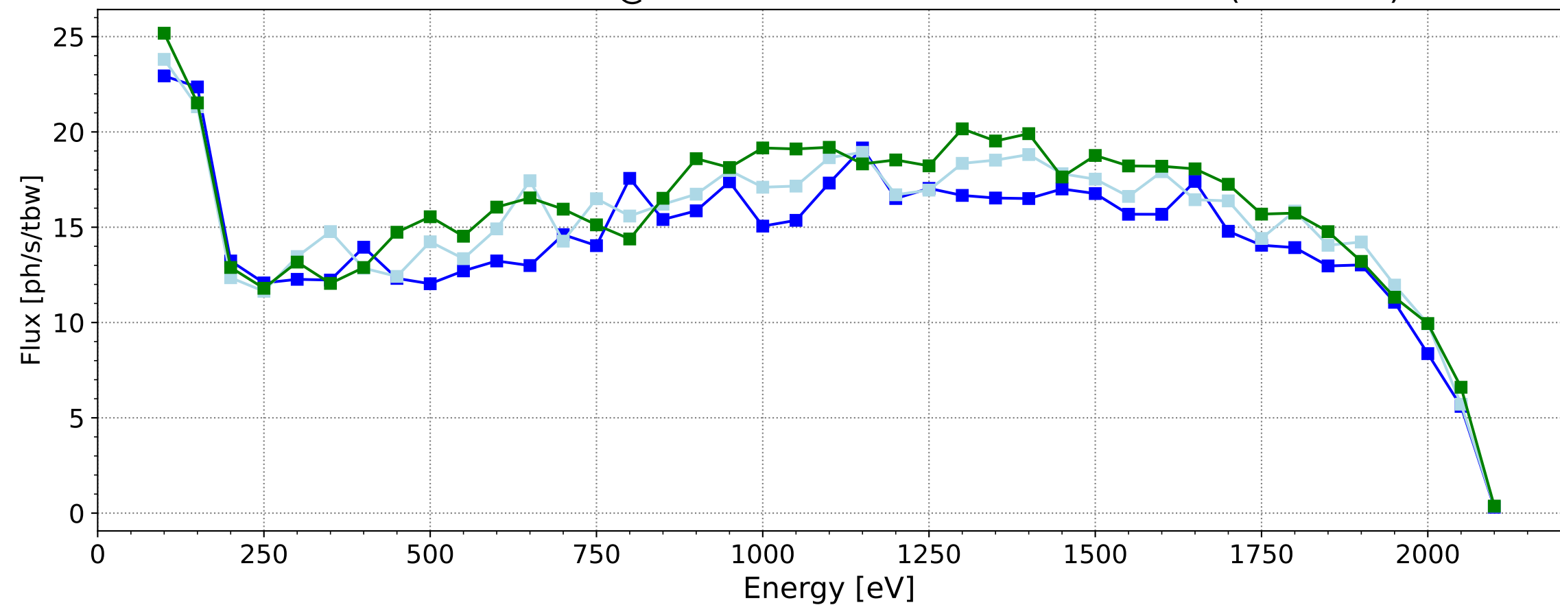
BESSY II vs. BESSY III @ 56 m standard PGM-BL PerMil flux (errors on)
